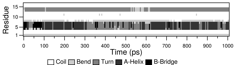
Fig. 5.58: Analysis of the secondary structure elements of a peptide in time.
