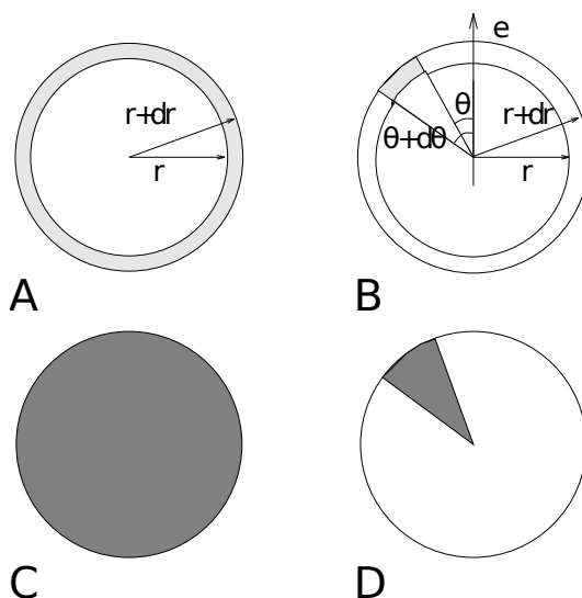
Fig. 5.50: Definition of slices in gmx rdf (page 135): A. g_{AB}(r) . B. g_{AB}(r, \theta) . The slices are colored gray. C. Normalization \langle \rho_B \rangle_{local} . D. Normalization \langle \rho_B \rangle_{local, \theta} . Normalization volumes are colored gray.
