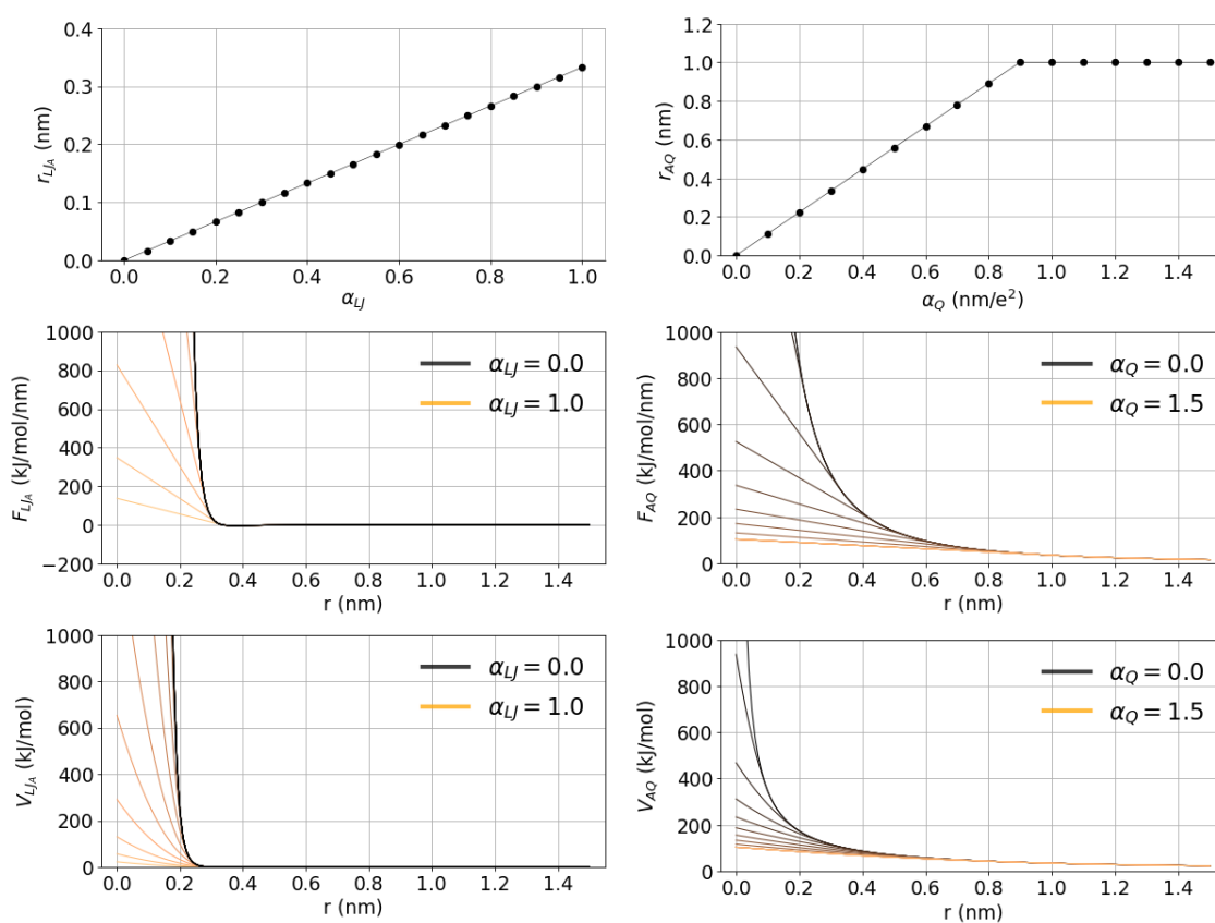
Fig. 5.33: Illustration of the soft-core parameter influence on the linearization point (top row), forces (middle row) and energies (bottom row) for van der Waals (left column) and electrostatic interactions (right column). The case of two interacting atoms is considered. In state A both atoms have charges of 0.5 and \sigma = 0.3 nm, \epsilon = 0.5 kJ/mol. In state B all the non-bonded interactions are set to zero. The parameter \lambda is set to 0.5 and electrostatic interaction cutoff is 1 nm.
