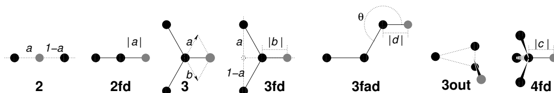
Fig. 5.35: The seven different types of virtual site construction. The constructing atoms are shown as black circles, the virtual sites in gray.
