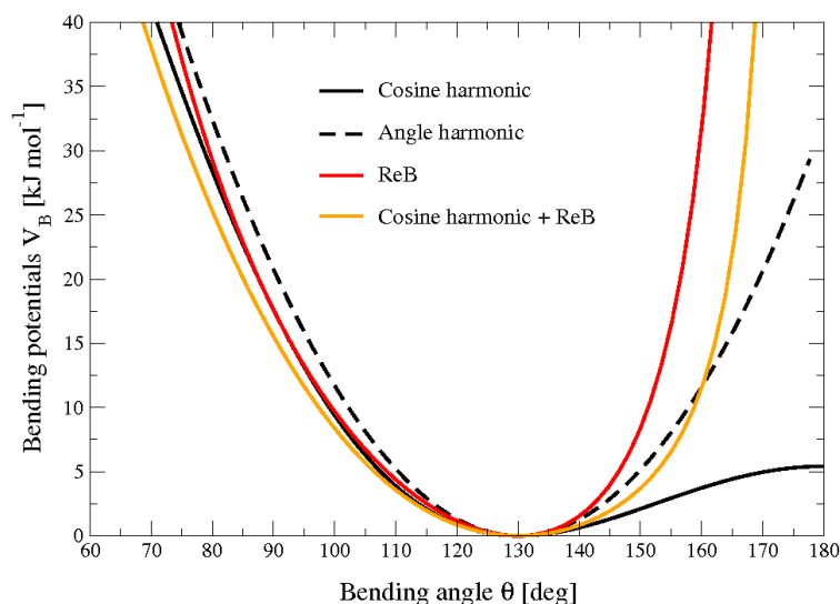
Fig. 5.22: Bending angle potentials: cosine harmonic (solid black line), angle harmonic (dashed black line) and restricted bending (red) with the same bending constant k_\theta = 85 \text{ kJ mol}^{-1} and equilibrium angle \theta_0 = 130^\circ . The orange line represents the sum of a cosine harmonic ( k = 50 \text{ kJ mol}^{-1} ) with a restricted bending ( k = 25 \text{ kJ mol}^{-1} ) potential, both with \theta_0 = 130^\circ .
