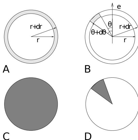
Fig. 5.52: Definition of slices in gmx rdf (page 291): A. g_{AB}(r) . B. g_{AB}(r, \theta) . The slices are colored gray. C. Normalization \langle \rho_B \rangle_{local} . D. Normalization \langle \rho_B \rangle_{local, \theta} . Normalization volumes are colored gray.
