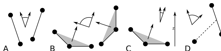
Fig. 5.56: Angle options of gmx gangle (page 223): A. Angle between two vectors. B. Angle between two planes. C. Angle between a vector and the z axis. D. Angle between a vector and the normal of a sphere. Also other combinations are supported: planes and vectors can be used interchangeably.
