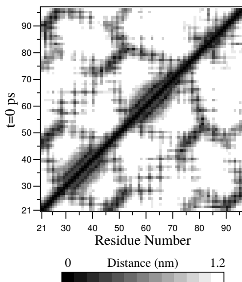
Fig. 5.57: A minimum distance matrix for a peptide 168 (page 690).
